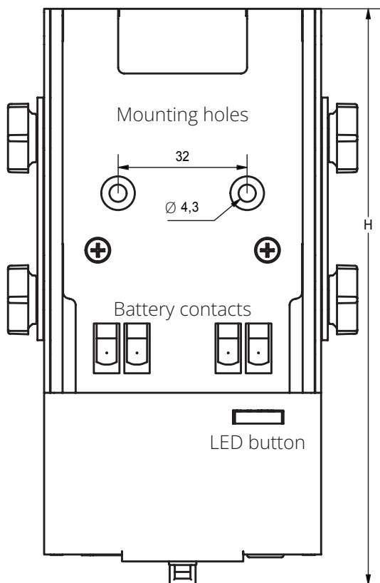
Cable tie holder
